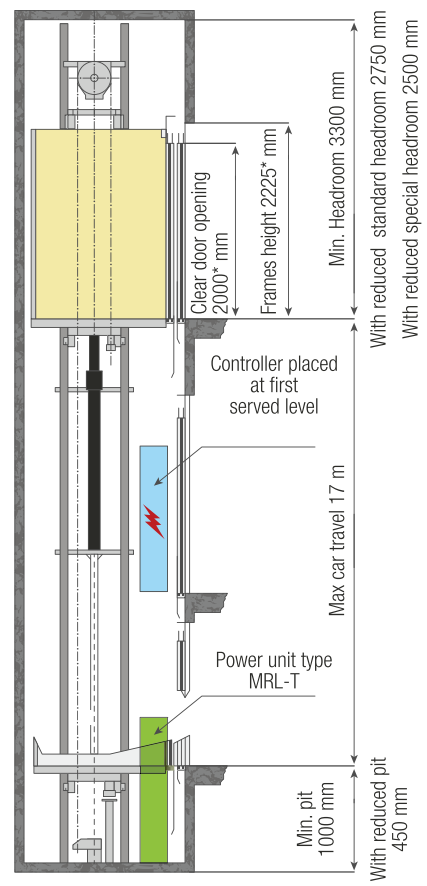
SHAFT SECTION
